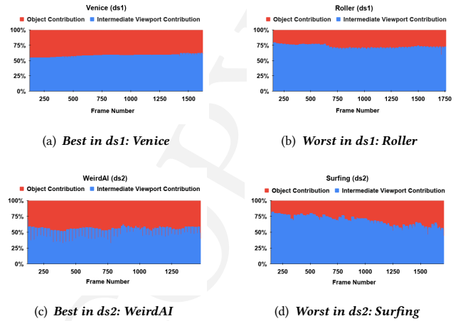
Figure 8: Percentage contribution of objects and past viewport in final prediction from PARIMA. Plots show the object contribution over the videos’ length having the best and worst average object contribution %.
